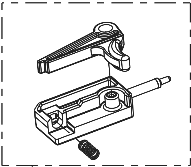
BOLT HANDLE ASSY. 169635-K00
