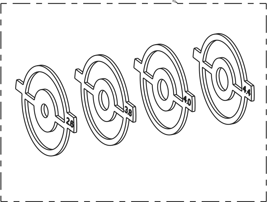
APERTURE INSERTS 168968-000
