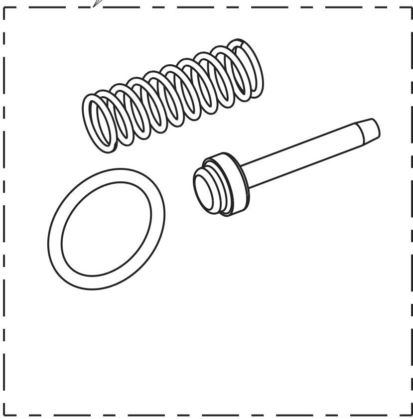
O-RING/VALVE GROUP 169766-K00
