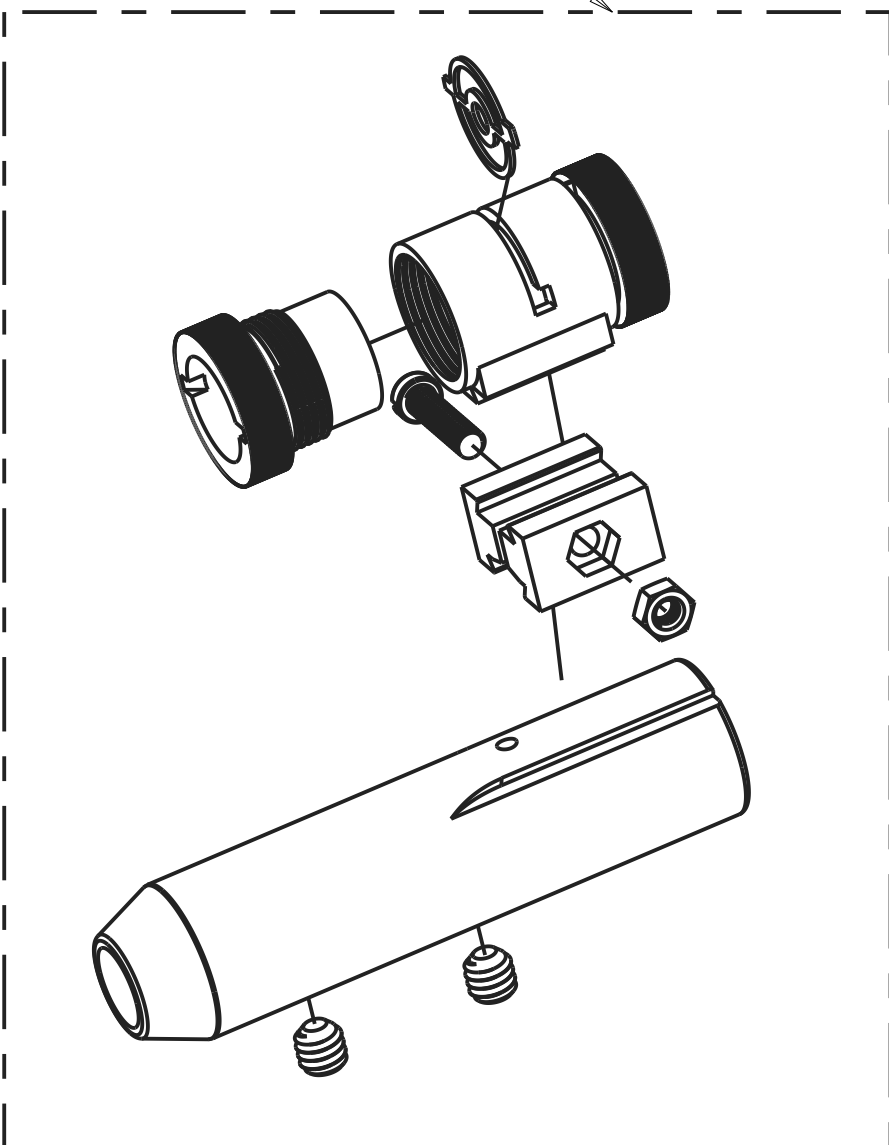
FRONT SIGHT BARREL WEIGHT ASSY. 168869-000
