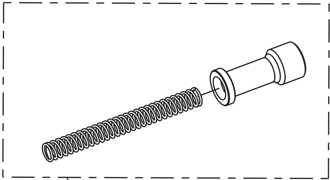
SAFETY ASSEMBLY 169318-K00
